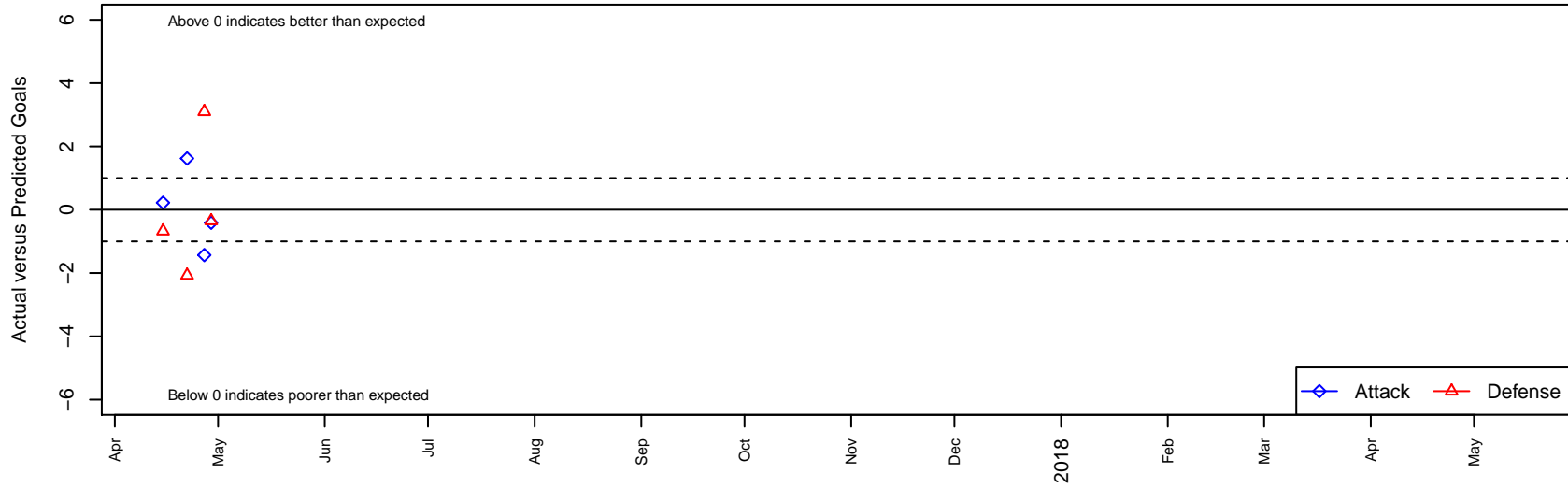
MSC Newman B05 Dots are actual minus expected GF (blue circles) and GA (red triangles). Blue line is smoothed change in attack strength. Red is smoothed change in defense strength.
